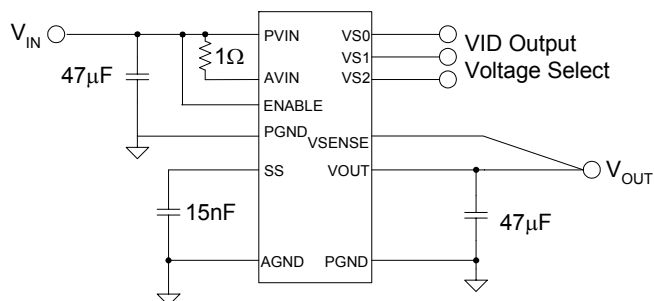
Figure 1. Simple Layout.
