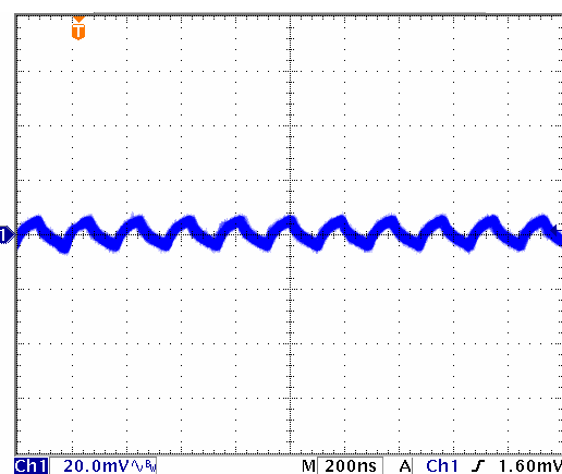
Ripple Voltage, 3.3V IN /1.2V OUT , I OUT =6A, C OUT = 5x10uF.
