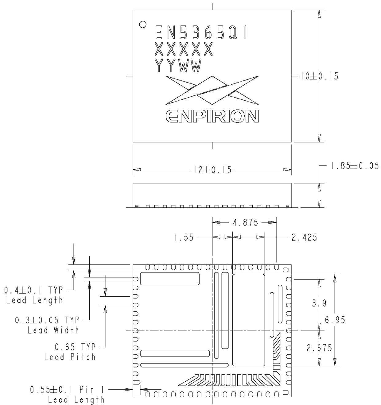
Figure 9. Package dimensions.
